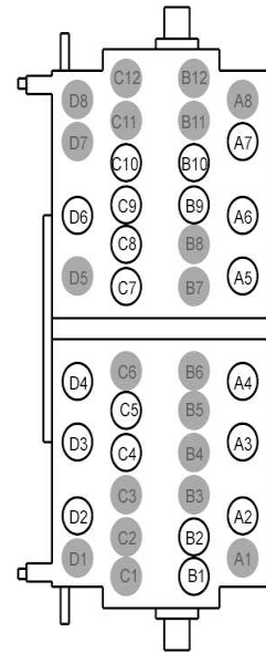
FEMALE Harness: 14A005
