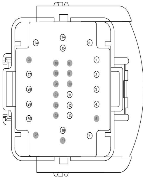
MALE Harness: 14401
